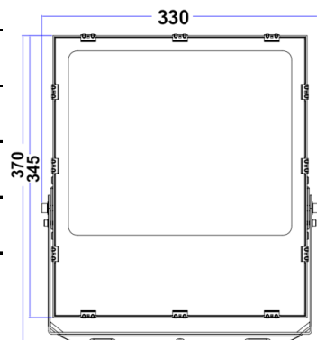
DIMENSION (mm)
