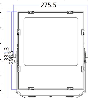
DIMENSION (mm)
